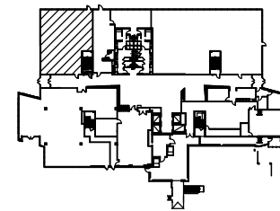
Key Plan - 1st Floor
